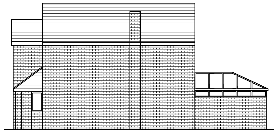
CONSERVATORY RIGHT FLANK AS PROPOSED (1:100)
