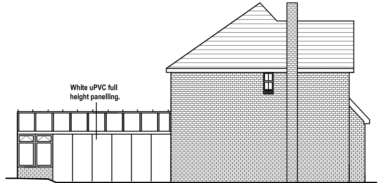
CONSERVATORY LEFT FLANK AS PROPOSED (1:100)
