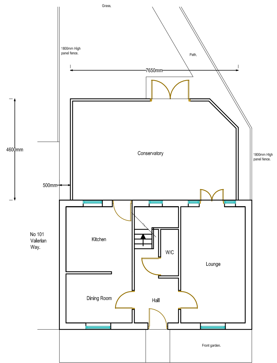
GROUND FLOOR PLAN AS PROPOSED (1:100)
