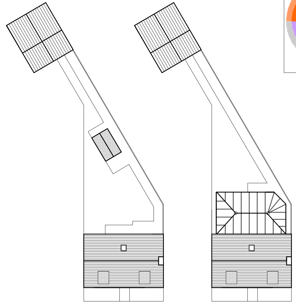
ROOF PLAN AS EXISTING (1:200)
