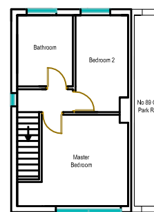
FIRST FLOOR PLAN AS EXISTING (1:100)
