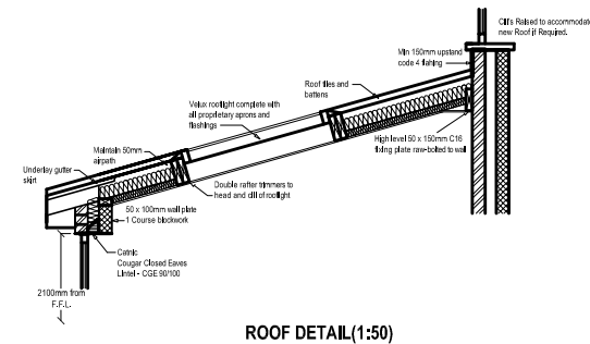
ROOF DETAIL(1:50)
