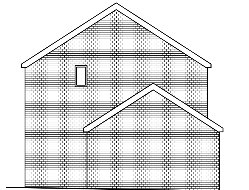
SIDE ELEVATION AS PROPOSED (1:100)
