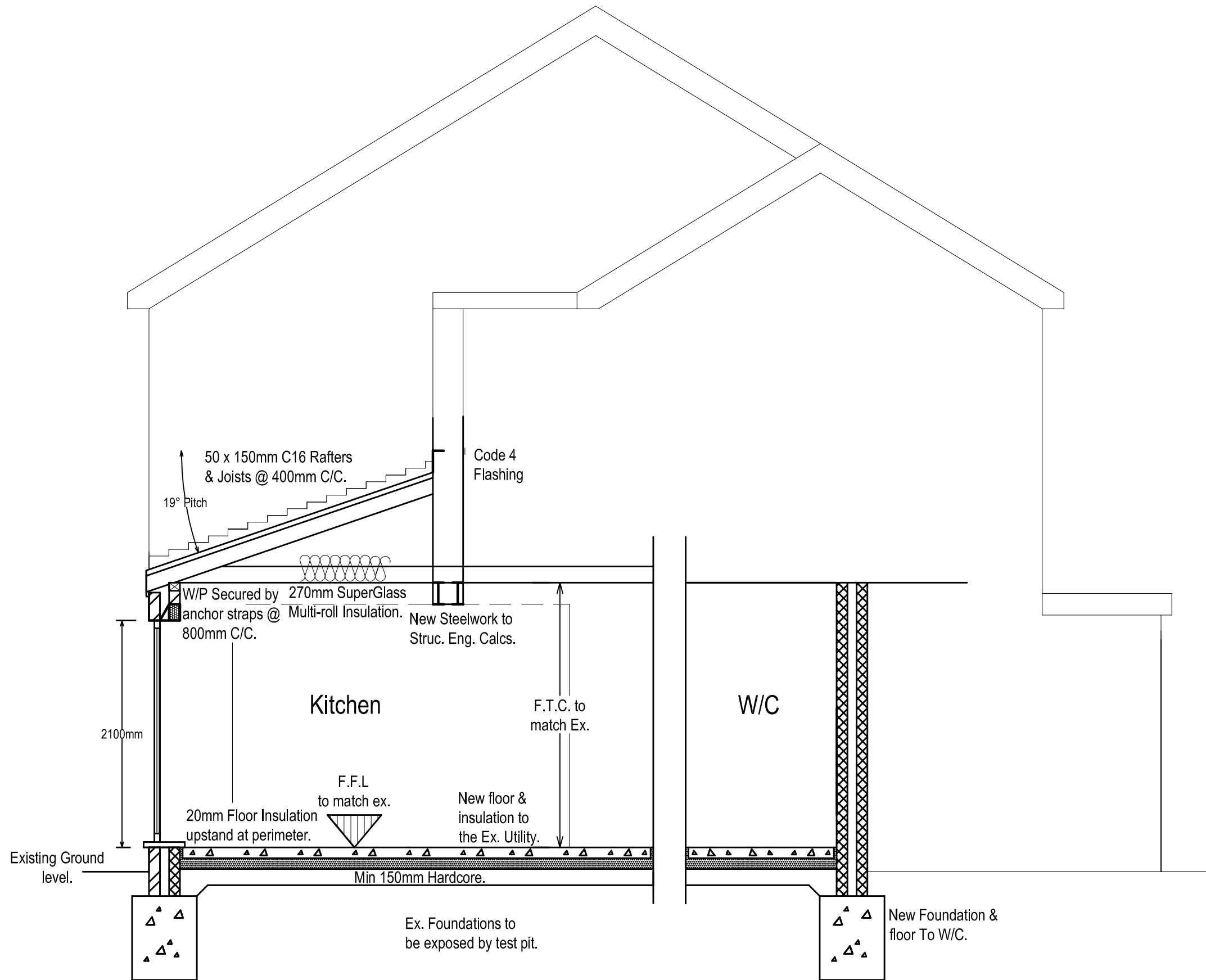
SECTION A-A (1:50)
