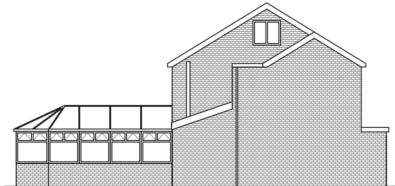
SIDE ELEVATION AS PROPOSED (1:100)
