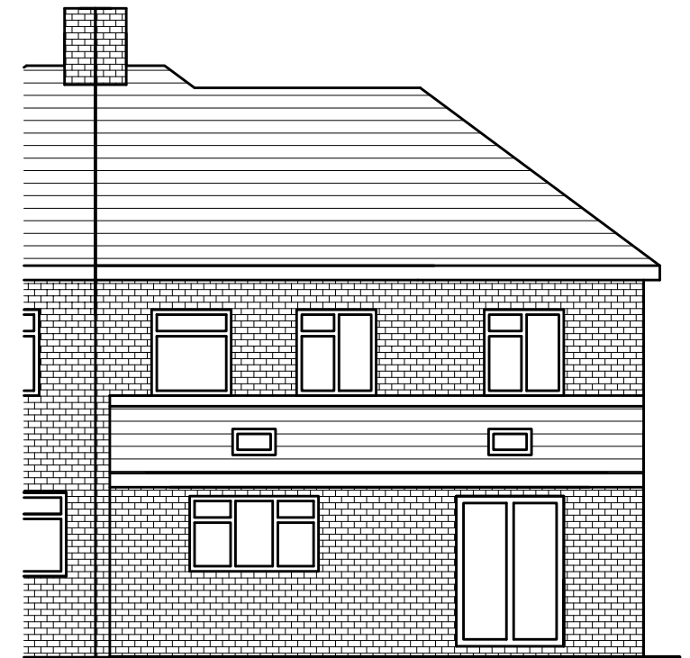
REAR ELEVATION AS PROPOSED (1:100)
